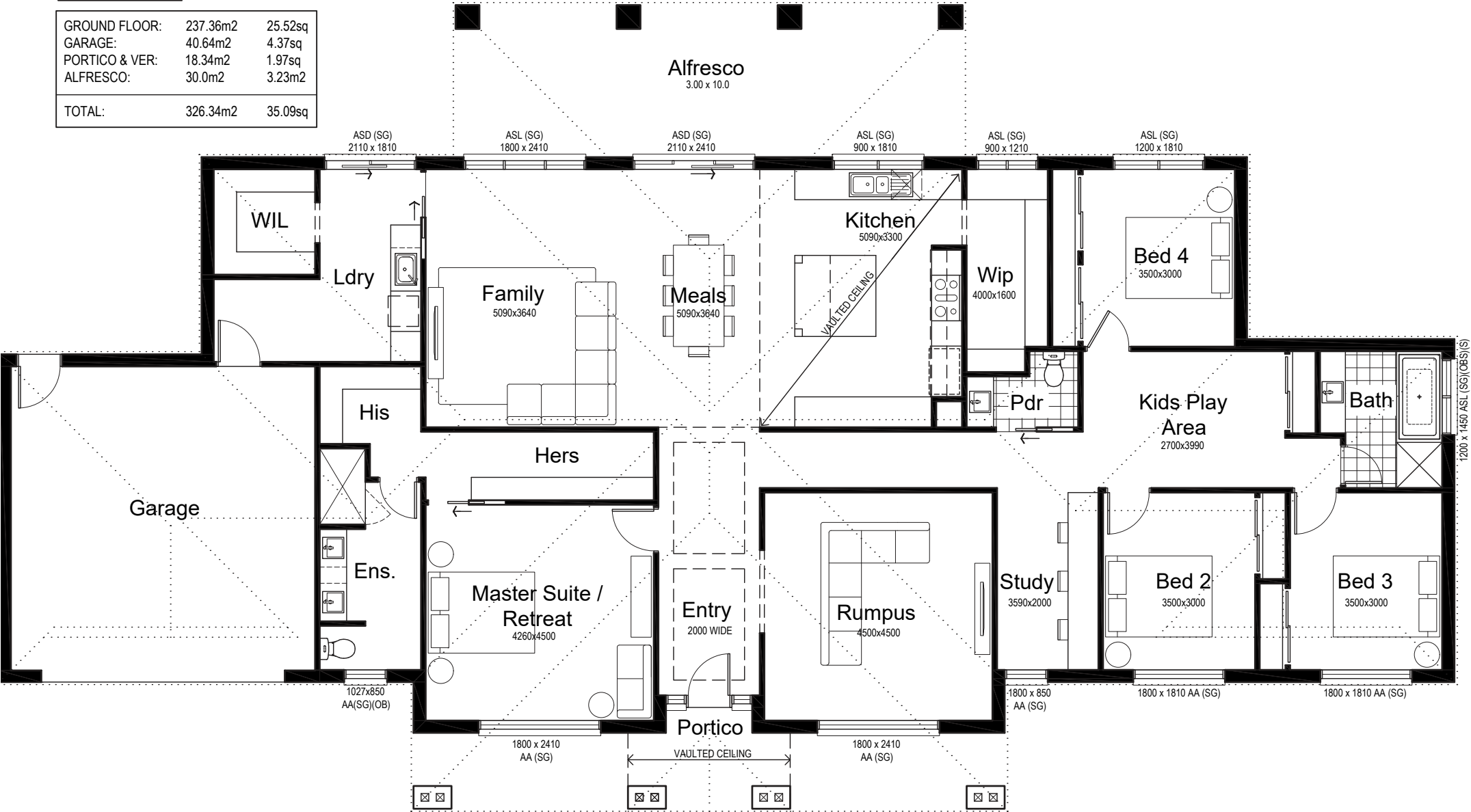
GROUND FLOOR 1:100 NOMINAL ROOM SIZES SHOWN
