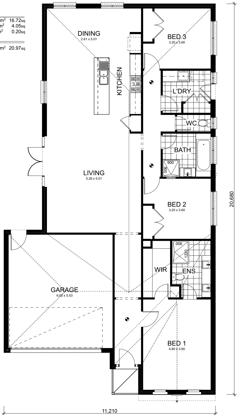
GROUND FLOOR mirrored 1:100 NOMINAL ROOM SIZES SHOWN
