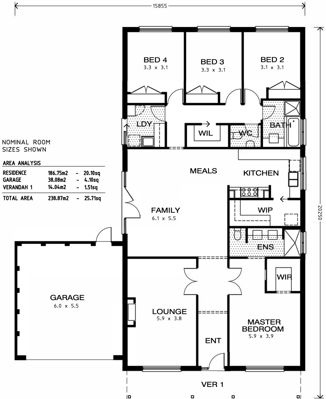
GROUND FLOOR 1:100 NOMINAL ROOM SIZES SHOWN
